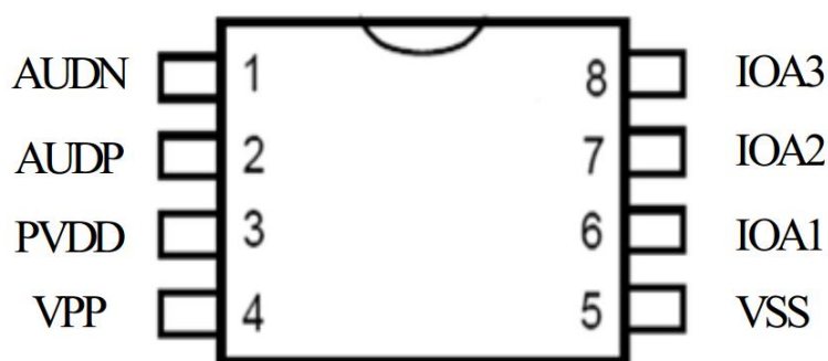
8 PIN SOP (150mil)
